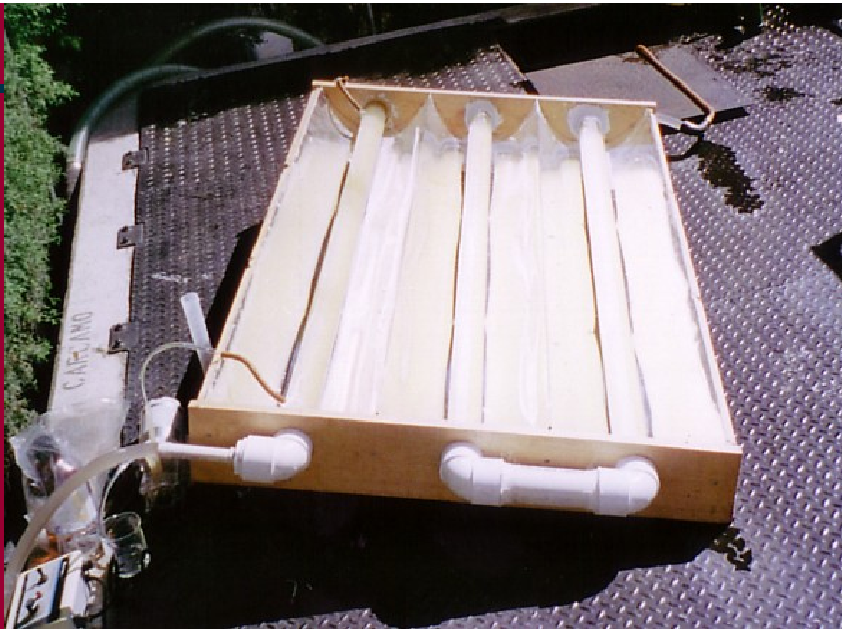
Home-made solar concentrator for R&D on treatment of industrial polluted water
