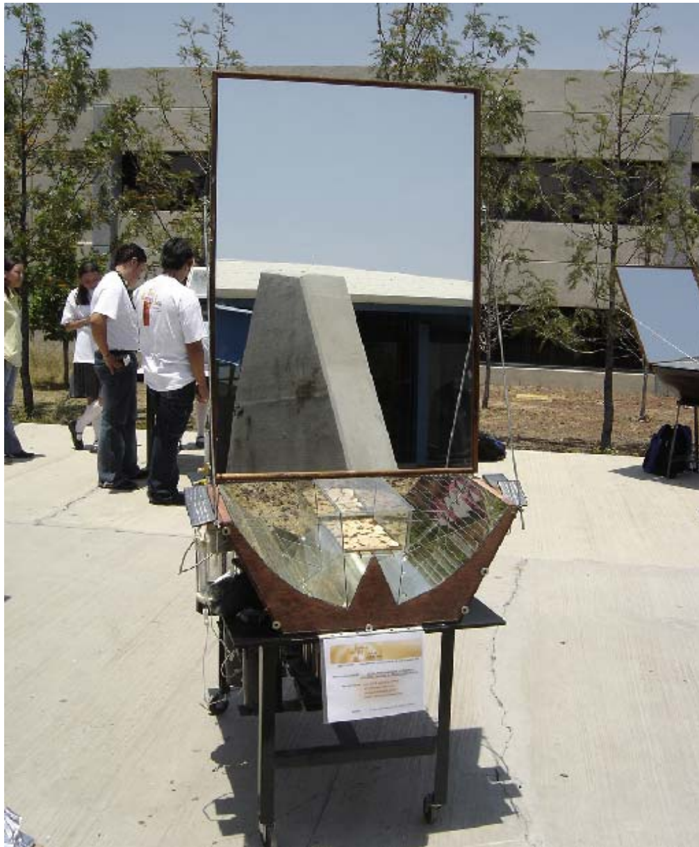
Tolokatsin 3 with solar refrigerator (photo to the right), and solar hot plate (photo to the left)
